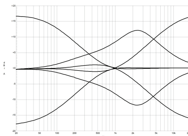
Illustration 2-16: HI, MID and LO filters
