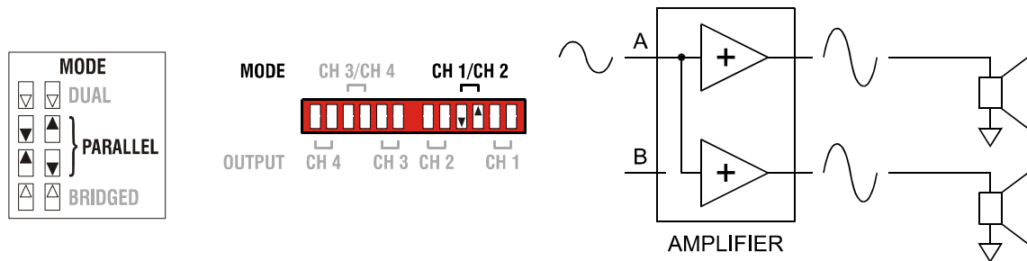
Illustration 2.2: Audio signal applied to input A connector in PARALLEL mode
