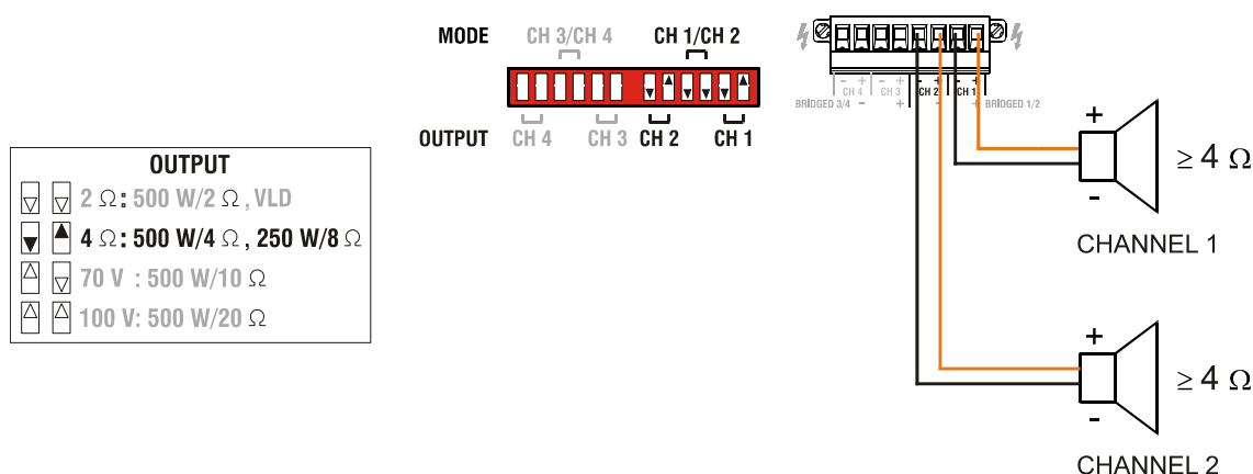
Illustration 2.5: DUAL mode of CH 1 and CH 2 in 4 Ohm Mode
