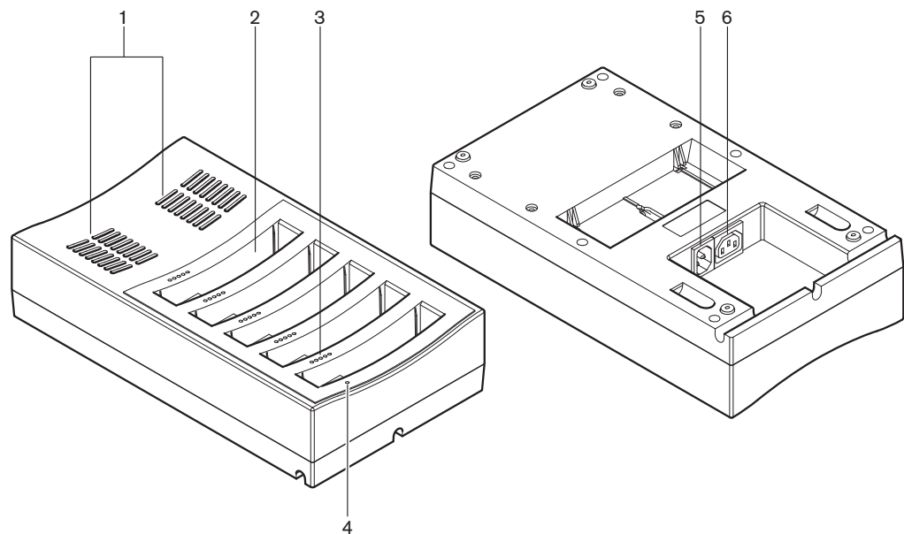
Figure 6.6: Chargeur DCNM-WCH05
