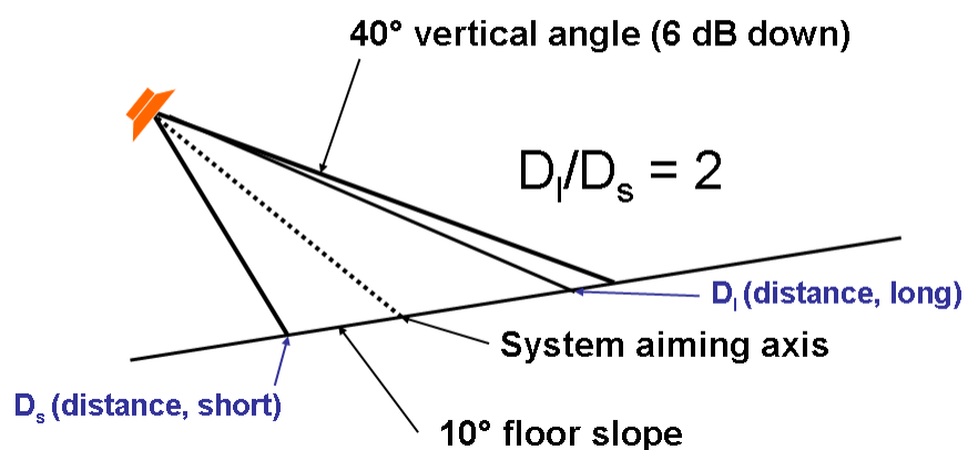
90° x 40° example, side view
