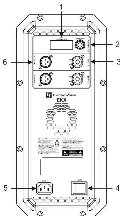
Figure 6.2: Panneau d'amplification du caisson sub-grave
