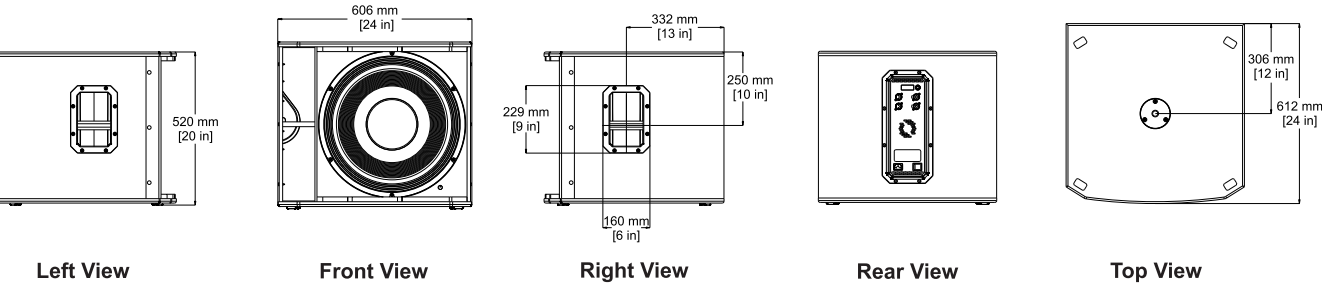
Figure 3.4: Dimensions du EKX-18SP
