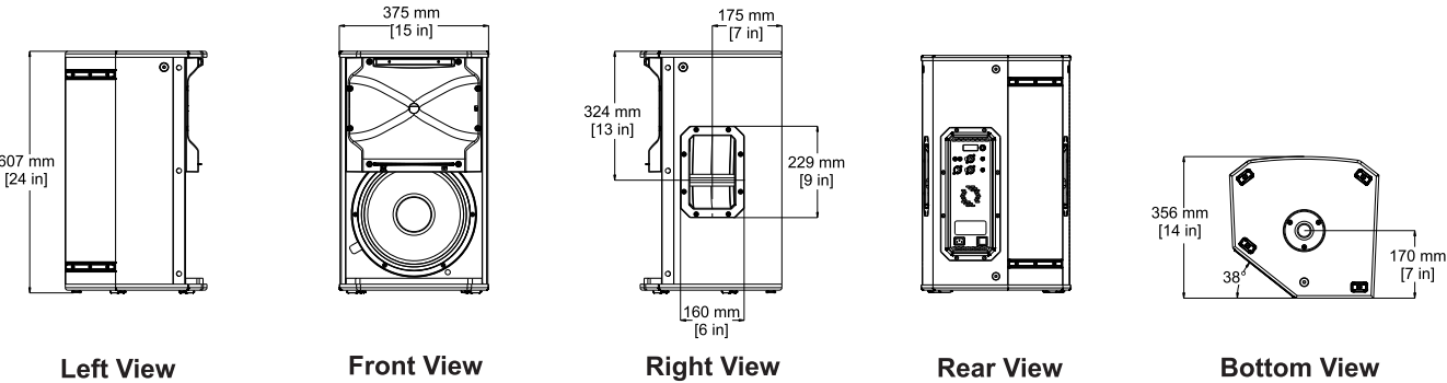
Figure 3.1: Dimensions du EKX-12P
