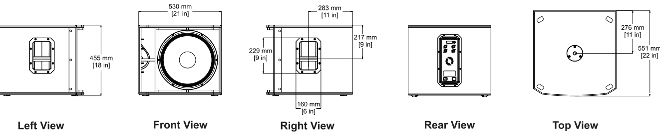
Figure 3.3: Dimensions du EKX-15SP
