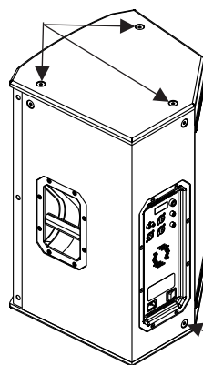
Figure 5.1: Points de suspension
