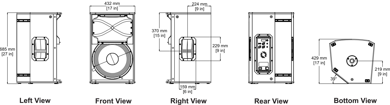
Figure 3.2: Dimensions du EKX-15P
