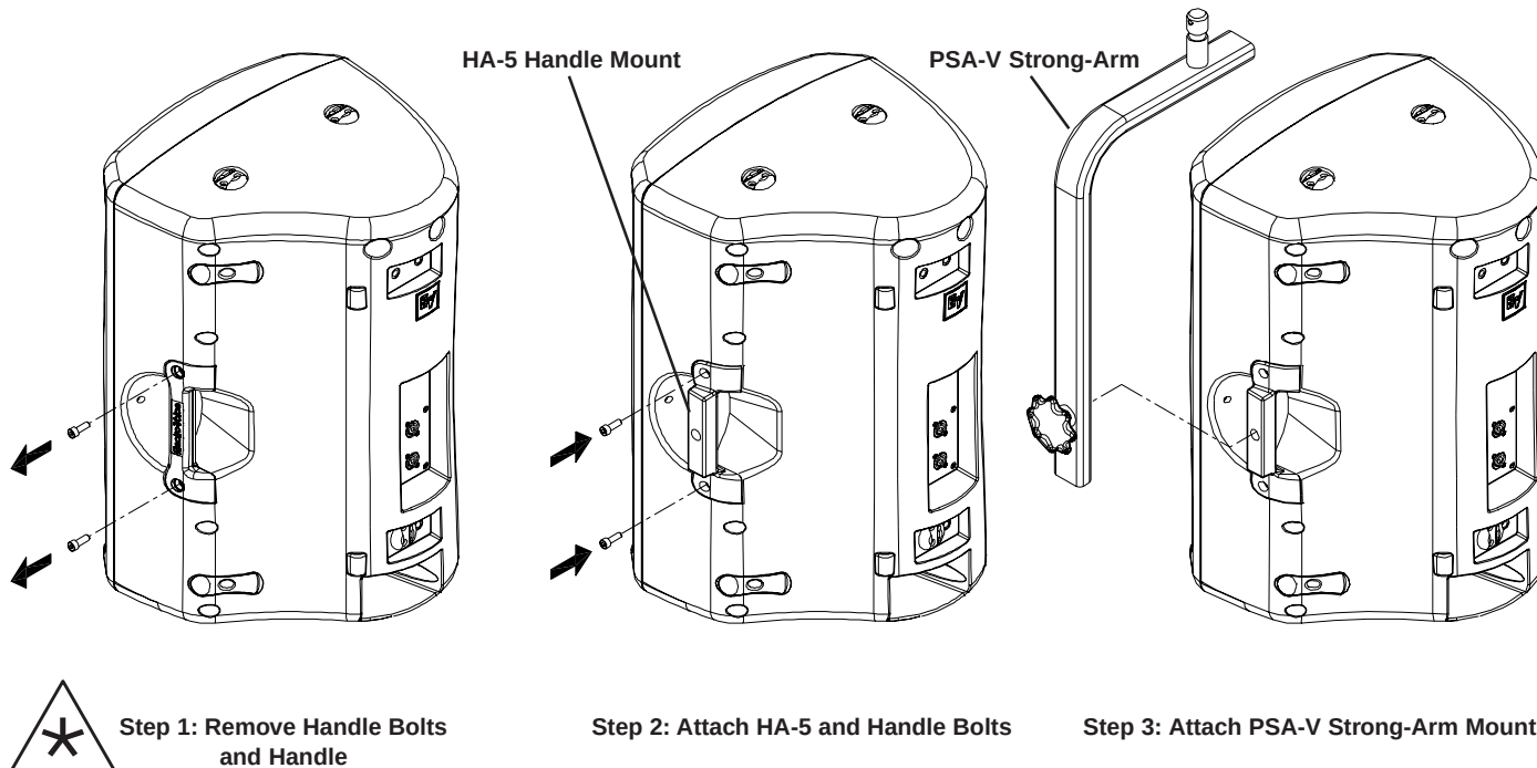
Figure 9: Assembling HA-5 Adapter for use with PSA-V Strong-Arm Mount Kits Used - HA-5 Handle Adapter Kit (x1) PSA-V Strong-Arm Mount (x1)
