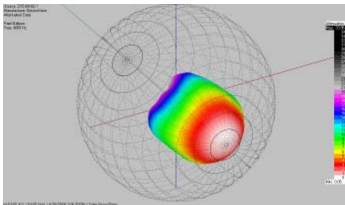
Figure 1a: 3D EASE Directivity Balloon, Zx5-60, 60° x 60° Coverage
