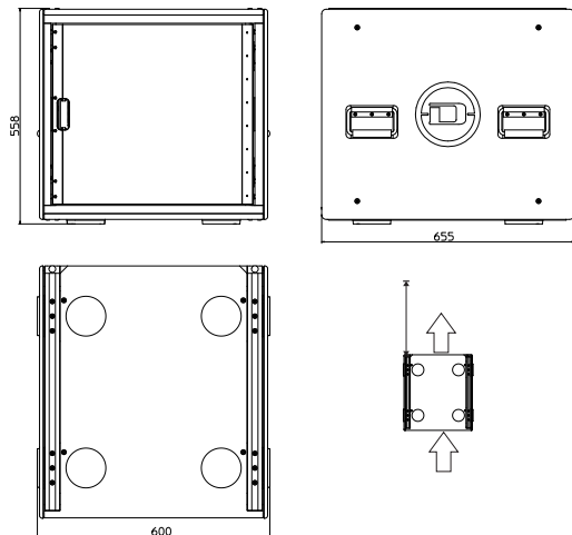
Dimensions: SR20TGX amplifier system rack
