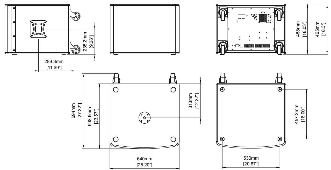
Illustration 1: Dimensions
